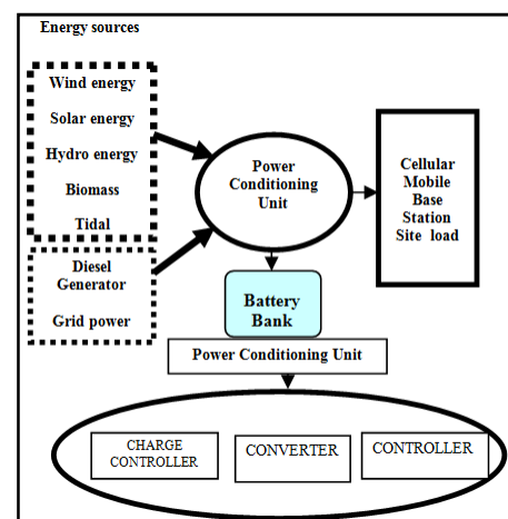
Fig. 1. Block Diagram of Hybrid Energy System for Cellular Mobile Telephony Base Station Site.
