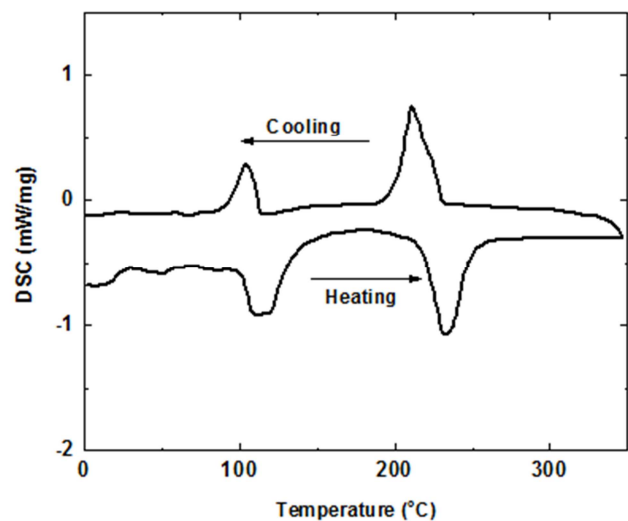
Figure 1. DSC thermogram record during heating and cooling of the eutectic system of ( \text{Na}_{0.6}\text{K}_{0.4} ) \text{NO}_3 sample.
